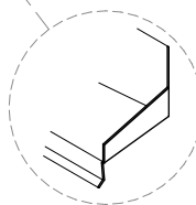
Stop-end tabbed up on both sides of head flashing
