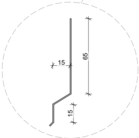
Standard 15mm head flashing
